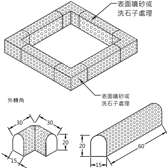
P14 預鑄洗石子(噴砂)樹穴
